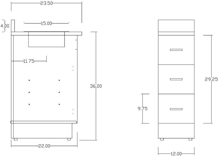
12 MEDICAL BASE CABINET 12 MEDICAL BASE CABINET — Side View & Front View (dimensions in inches)
