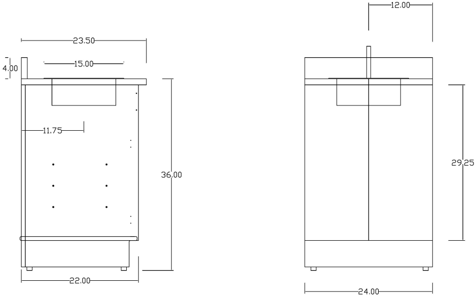
24 MEDICAL BASE CABINET 24 MEDICAL BASE CABINET — Side View & Front View (dimensions in inches)
