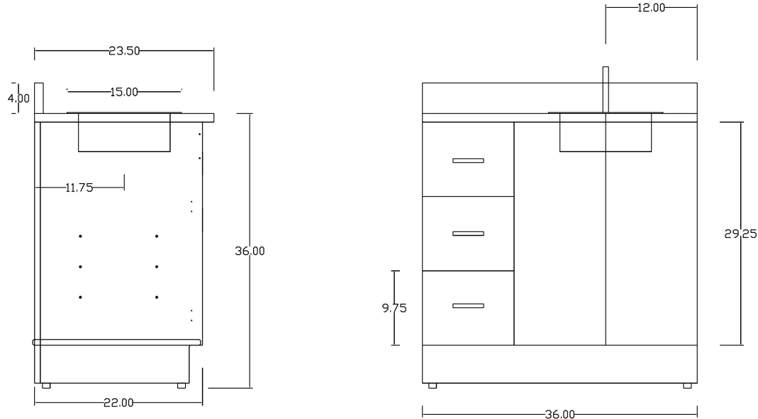
36 MEDICAL BASE CABINET 36 MEDICAL BASE CABINET — Side View & Front View (dimensions in inches)
