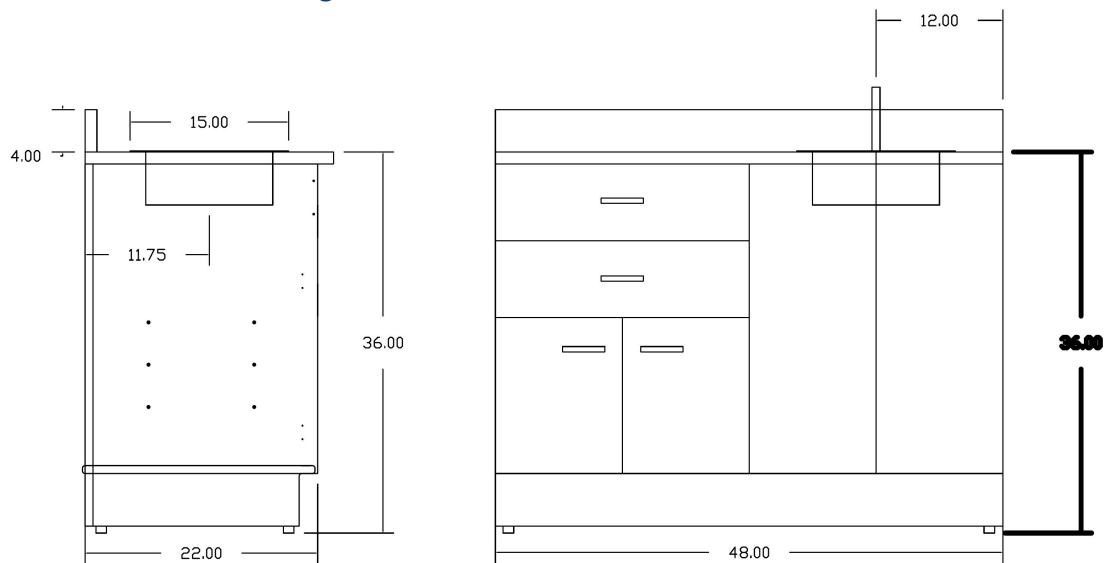
48" MEDICAL BASE CABINET 48" MEDICAL BASE CABINET — Side View & Front View (dimensions in inches)
