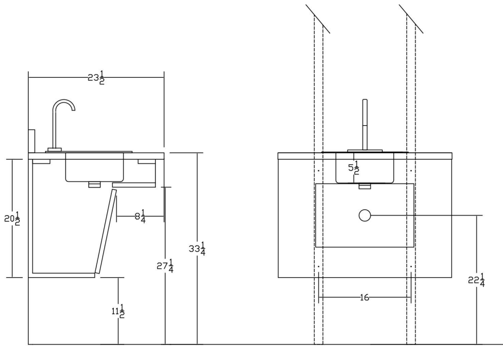
ADA SINK VANITY DIMENSIONS ADA SINK VANITY DIMENSIONS — Side View & Front View (dimensions in inches)
