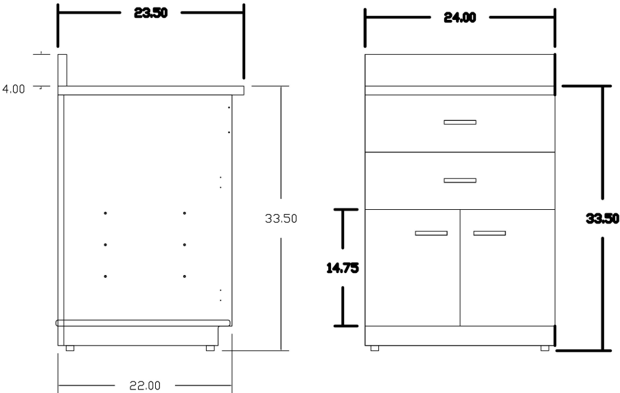
ADA BASE CABINET 24" 2 DRAWERS ADA BASE CABINET 24" 2 DRAWERS — Side View & Front View (dimensions in inches)
