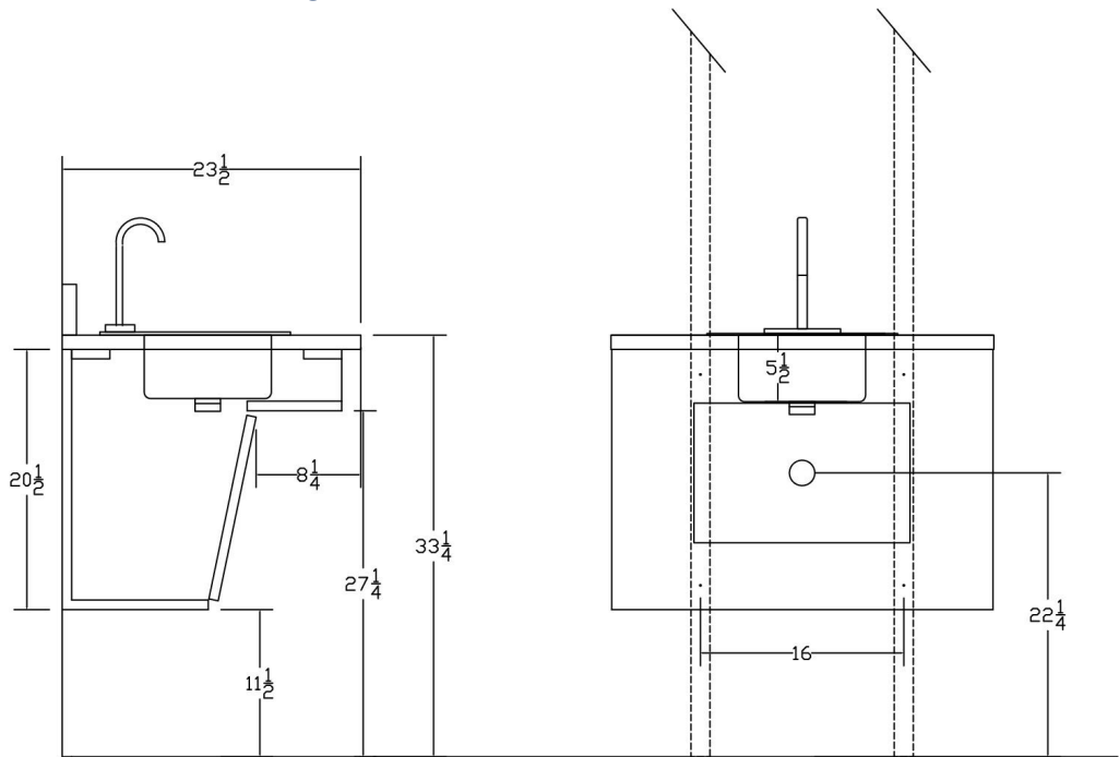
ADA SINK VANITY DIMENSIONS ADA SINK VANITY DIMENSIONS — Side View & Front View (dimensions in inches)
