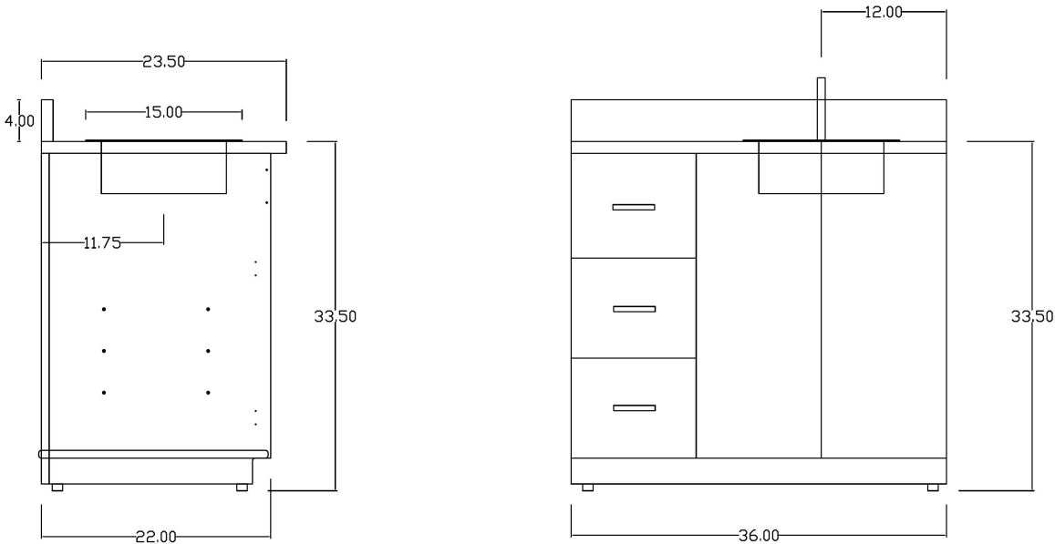
ADA BASE CABINET 36 DRAWERS ADA BASE CABINET 36 DRAWERS — Side View & Front View (dimensions in inches)
