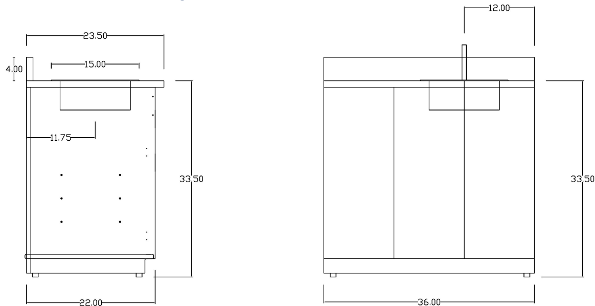
ADA BASE CABINET 36 DOORS ADA BASE CABINET 36 DOORS — Side View & Front View (dimensions in inches)
